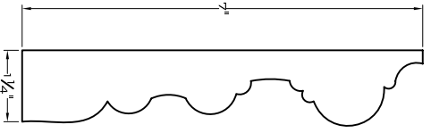
# 12 -BASEBOARD- -A-B-7"
