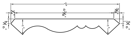
# 18 CROWN -D-7"
